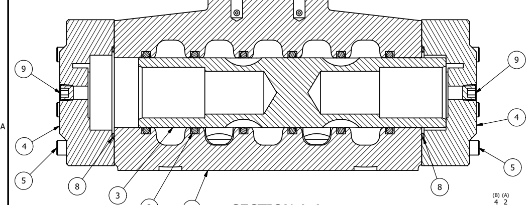
SECTION A-A SCALE 1/2 VIEW FROM 3 PORT SIDE
