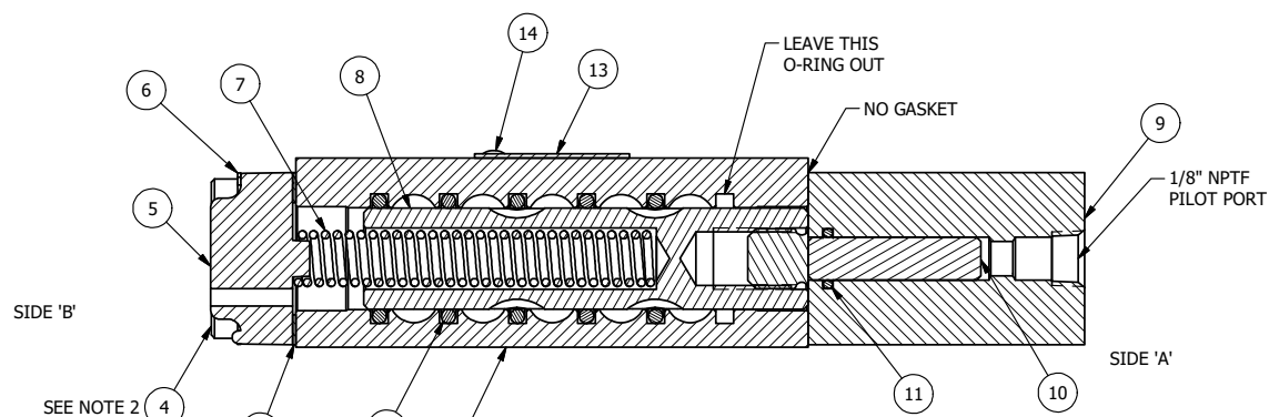
SECTION A-A SCALE 1 : 1 VIEW FROM 3 PORT SIDE
