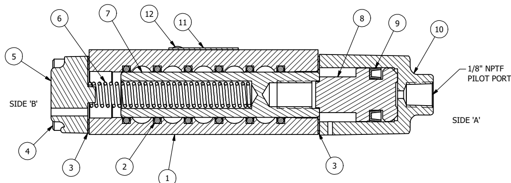
SECTION A-A SCALE 1 : 1 VIEW FROM 3 PORT SIDE
