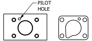
POSITION GASKET TO SEAL PILOT HOLE BOTH SIDES. (SIDE 'A' SHOWN)
