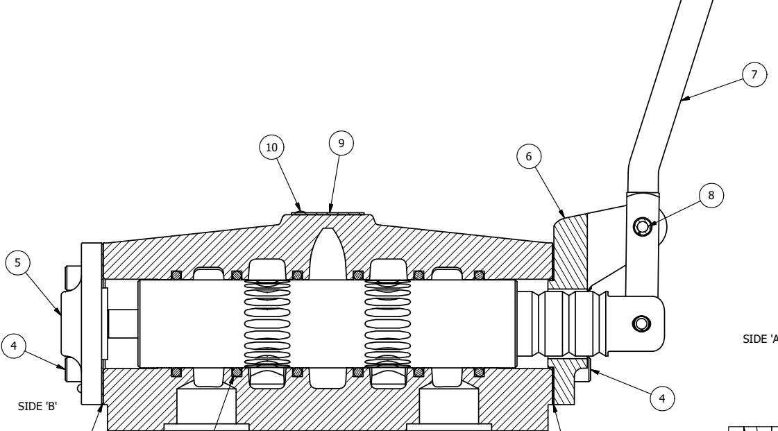
SECTION A-A SCALE 3/4 VIEW FROM 3 PORT SIDE
