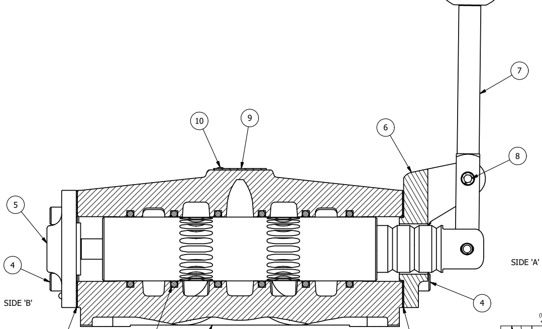
SECTION A-A SCALE 3/4 VIEW FROM 3 PORT SIDE
