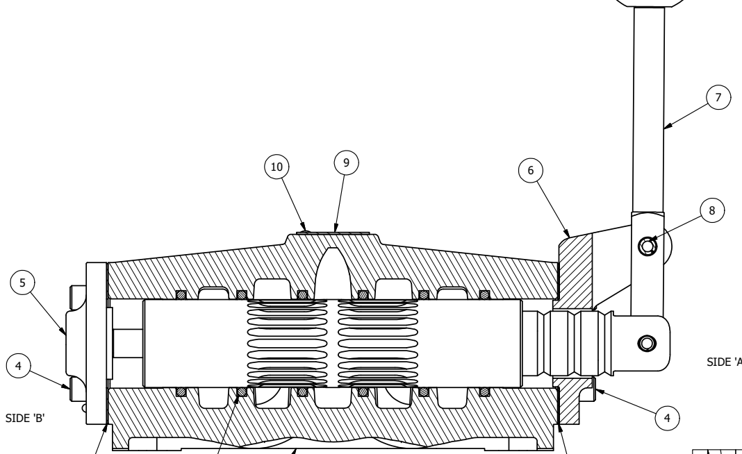
SECTION A-A SCALE 3/4 VIEW FROM 3 PORT SIDE
