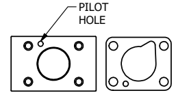
POSITION GASKET TO SEAL PILOT HOLE BOTH SIDES. (SIDE 'A' SHOWN)
