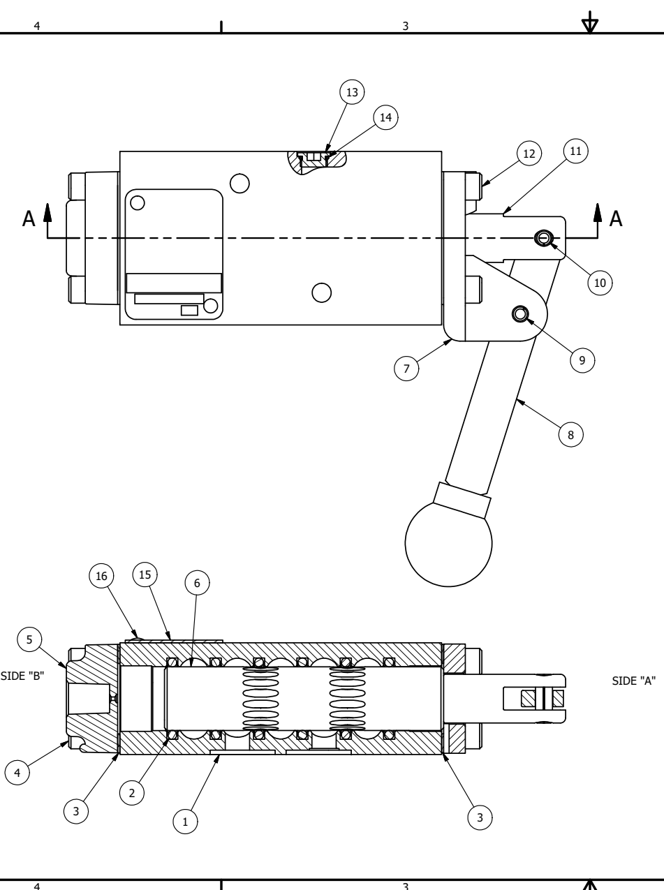
SECTION A-A SCALE 1 : 1 VIEW FROM 3 PORT SIDE
