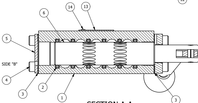
SECTION A-A SCALE 1 : 1 VIEW FROM 3 PORT SIDE
