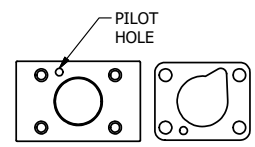
POSITION GASKET TO SEAL PILOT HOLE BOTH SIDES. (SIDE 'A' SHOWN)
