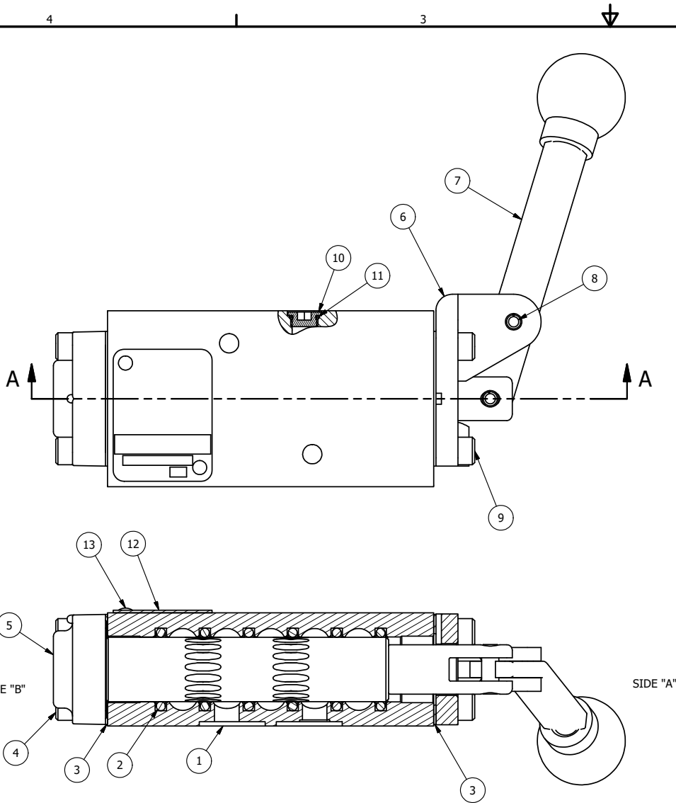
SECTION A-A SCALE 1 : 1 VIEW FROM 3 PORT SIDE
