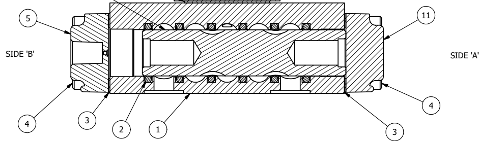
SECTION A-A VIEW FROM 3 PORT SIDE
