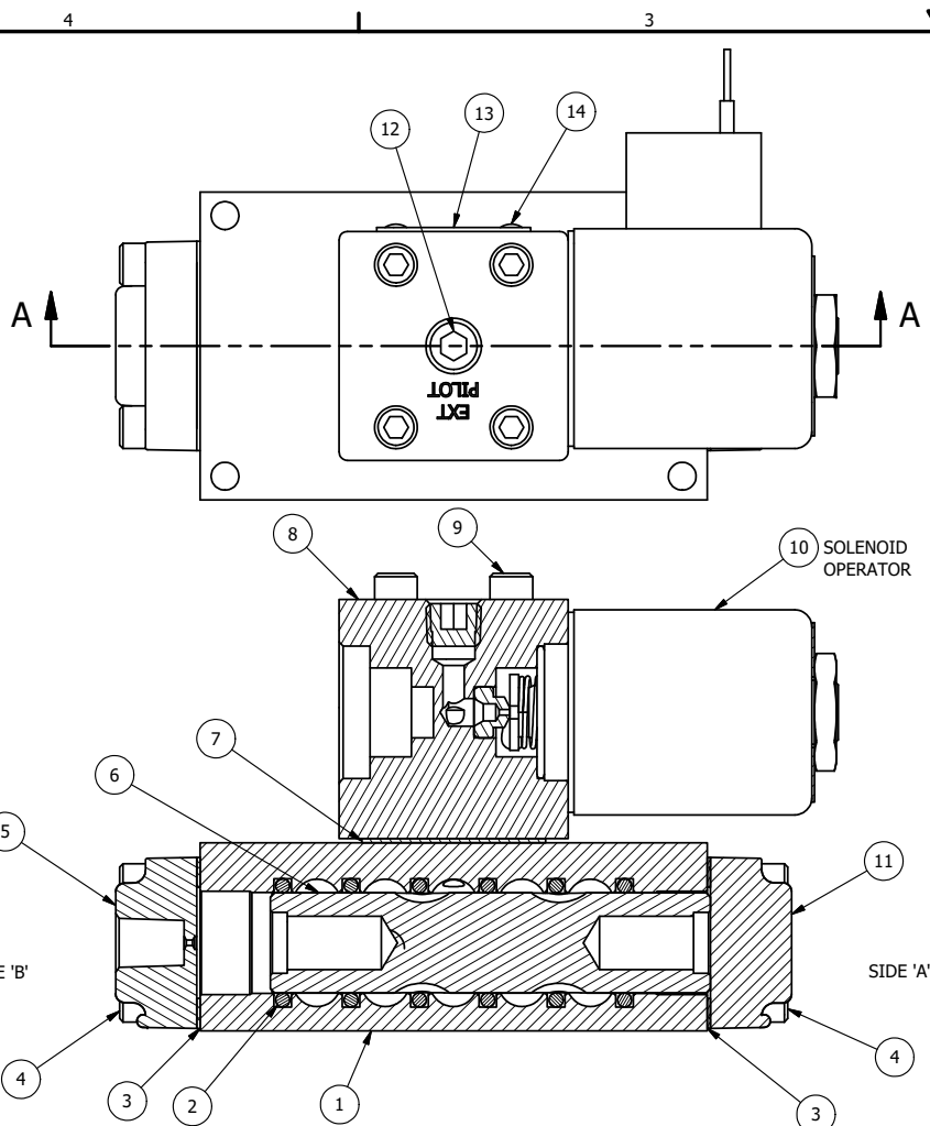
SECTION A-A VIEW FROM 3 PORT SIDE
