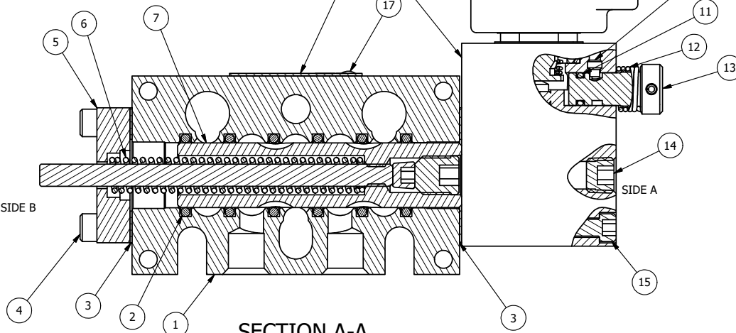
SECTION A-A VIEW FROM O-RING SIDE
