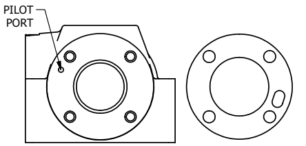
POSITION GASKET TO SEAL PILOT HOLE ON BOTH SIDES ('A' SHOWN)
